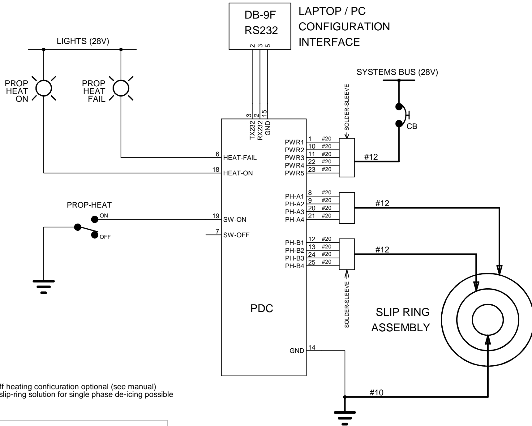
Typical PDC Electrical Installation
